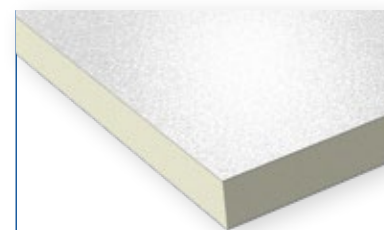
Polyiso Foam Dimensions: 600 x 1200 mm Facers: Embossed aluminium of 50 \mu m Resistance to vapor factor \mu = \infty
